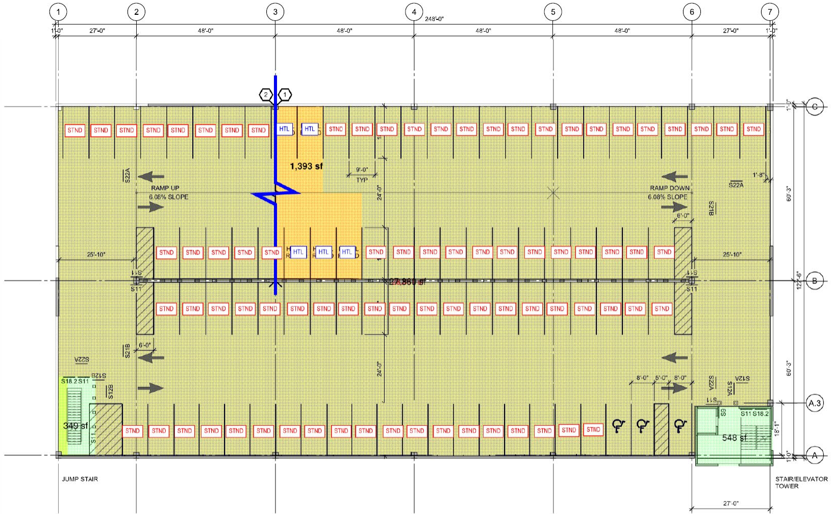
2 LEVEL 2 PLAN 1/16" = 1'-0"
